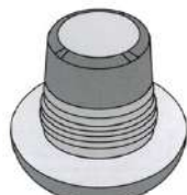
30761 Unit Pump Tappet UIS (PDE) Total items 60 pcs. - 12 tappet size from 14,56 to 14,78 mm (cut 0,02)
