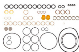
33295 094040-0030 for HP0 pump (John Deere series 20)
