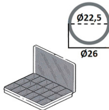
15140 Shim Kit \varnothing 26 - Hole \varnothing 22,5 Total items 240 pcs. – 24 shims size from 2,04 to 2,50 (cut 0,02)
